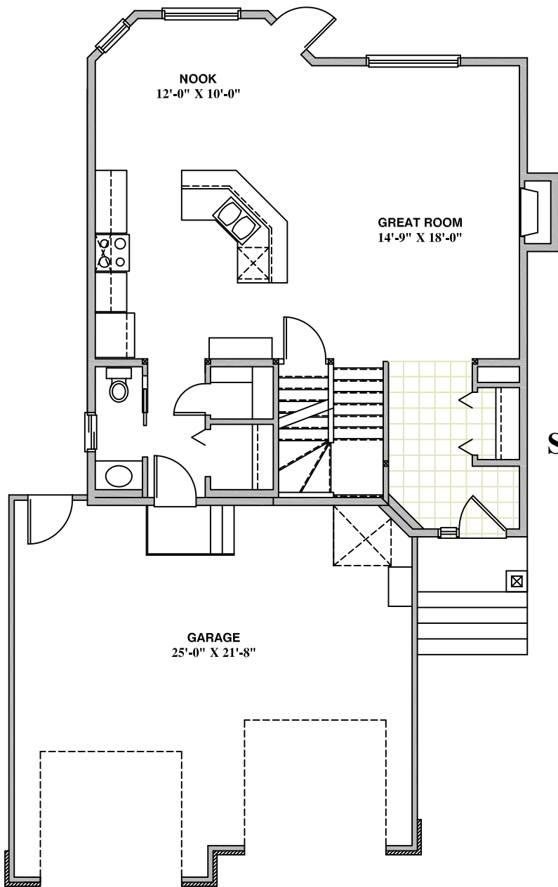
MAIN FLOOR 793 Sq. Ft.
